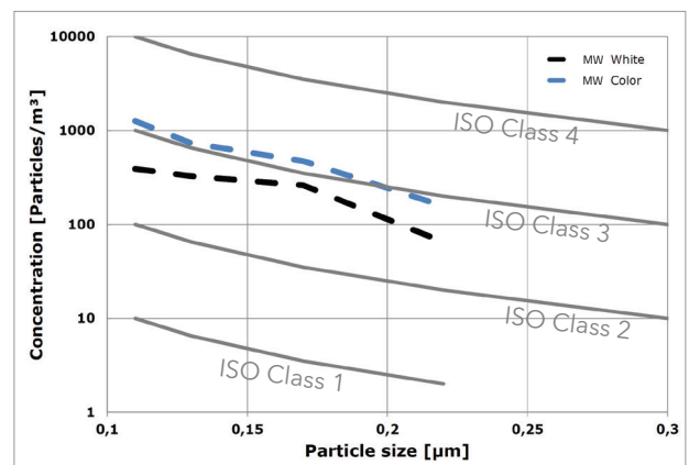
Figure 1: Test results for cleanroom KE fabrics
