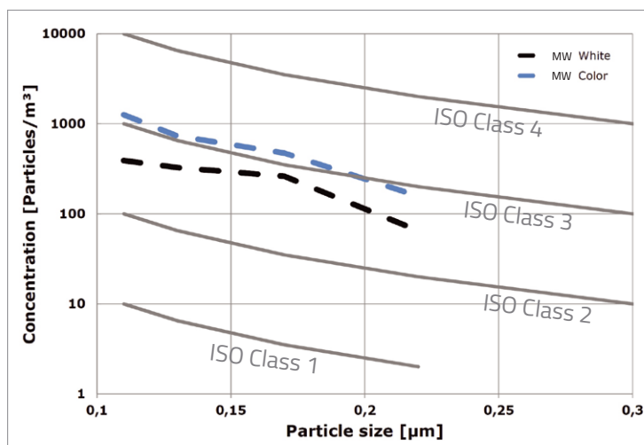
Figure 1: Test results for cleanroom KE Textile materials
