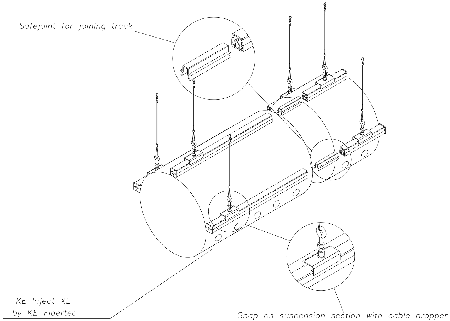
Triple Track Suspension Detail for KE Fibertec Fabric Ducts (3, 9 & 12 O'clock Attachment)
