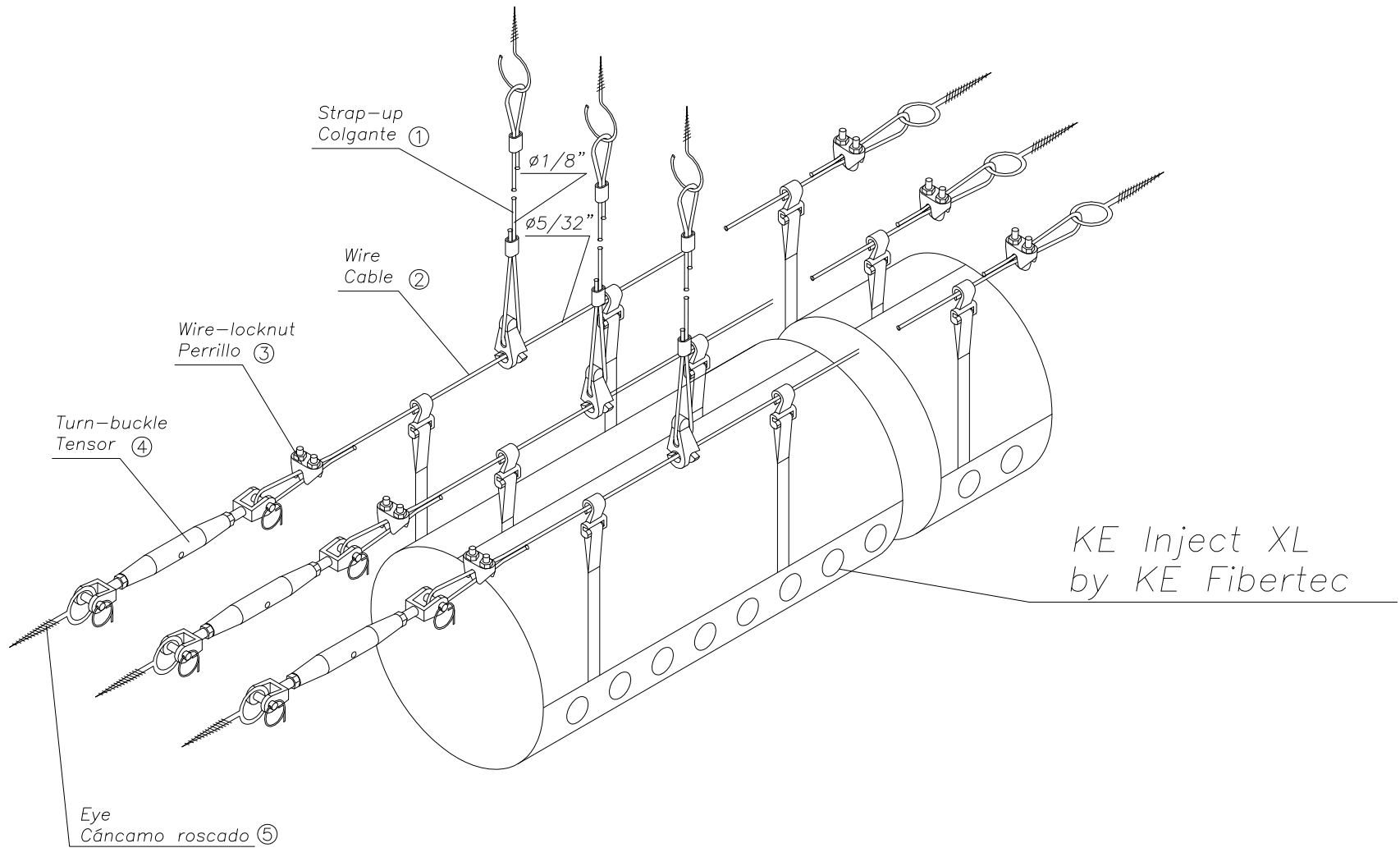
Triple Cable Suspension Detail for Fabric Ducts (12 o' clock Attachment)
