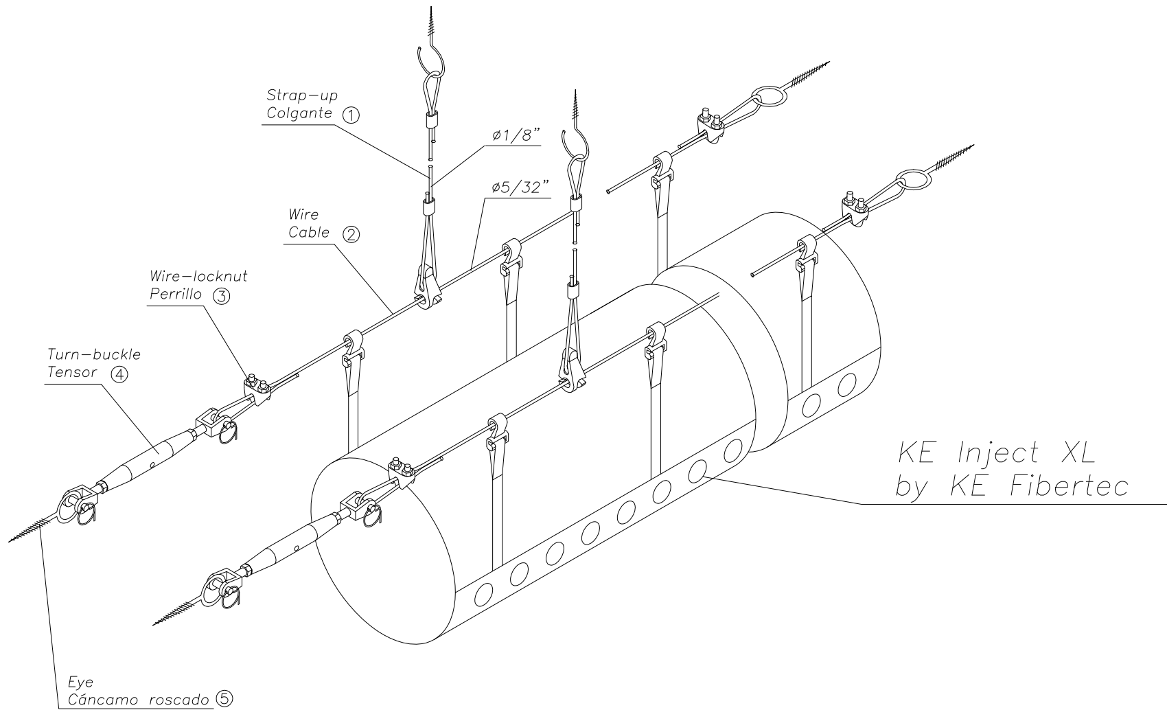
Double Cable Suspension Detail for Fabric Ducts (12 o' clock Attachment)
