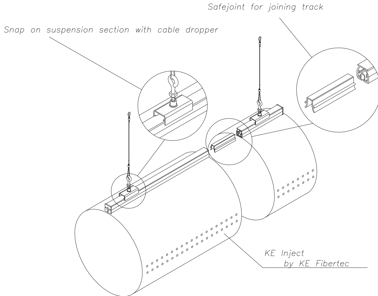
Single Track Suspension Detail for KE Fibertec Fabric Ducts (12 o' clock Attachment)
