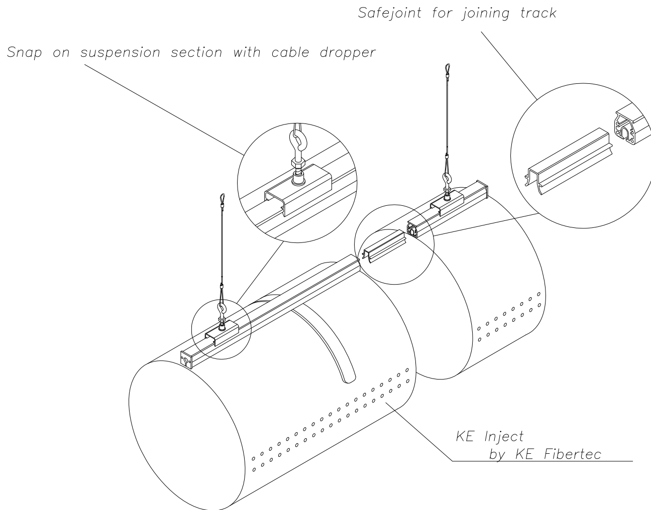
Safetrack Arch Suspension Detail for KE Fibertec Fabric Ducts (12 o' clock Attachment)
