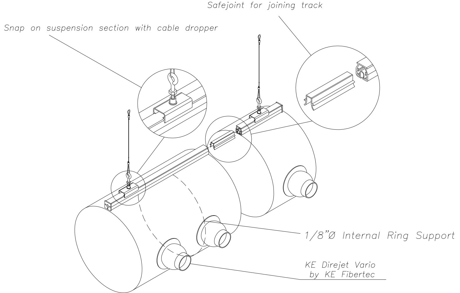
Safetrack 360° Suspension Detail for KE Fibertec Fabric Ducts (12 o'clock Attachment)
